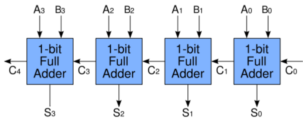
图 14.2. 4-bit Ripple Carry Adder
